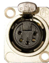
XLRF4-D 4-pin XLR female Neutrik® NC4FDL-1
